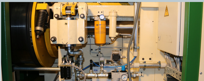
Pneumatic System - Lubrication
